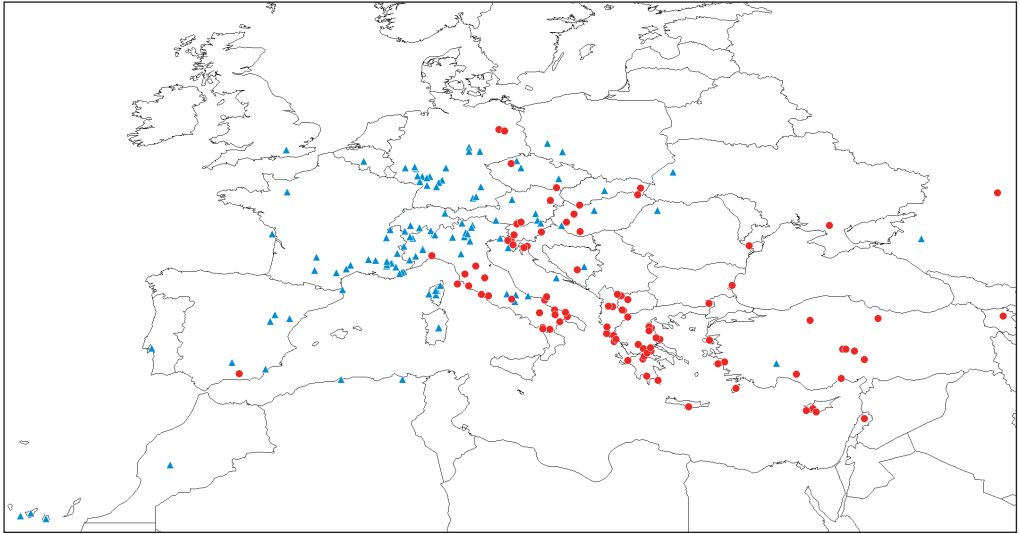
Fig. 36. Distribution map of Cephimallota angusticostella (red circles) and C. crassiflavella (blue triangles) in the West Palaearctic.
