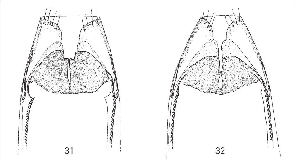
Figs 31–32. C. crassiflavella , ♀ genitalia (with variability): 31. Wroclaw [labelled: Breslau, 1896], Poland; 32. Bocognano, Corsica, France.
